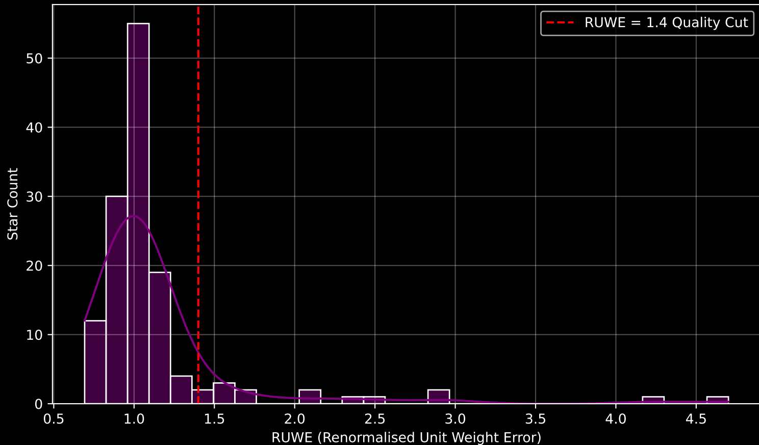
GAPOGEE DR17 Field [282-37-O_TESS] RUWE Distribution (n= 135)
